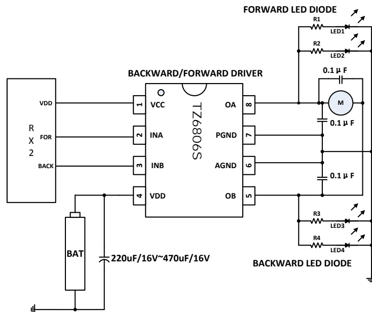
Fig. 3 Schematic diagram for remote controlled toy car LED indicator connection
